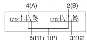
Distributeur 2x4/2, 3 orifices (C)
