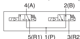
Distributeur 2x4/2, 3 orifices (C)
