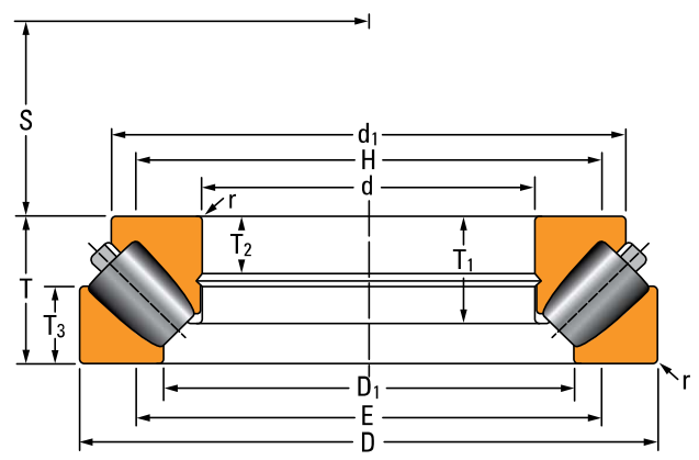
Type TSR-EM
