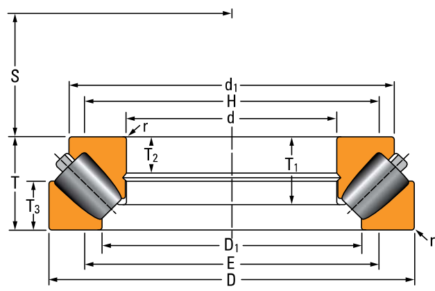
Type TSR-EM
