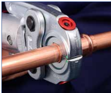
5. Complete joint with the press tool
