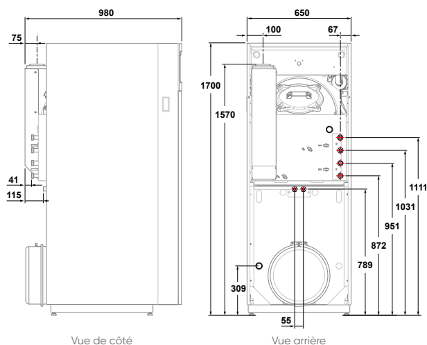
Axeo NOx Duo F07 / Axeo NOx Duo F30
