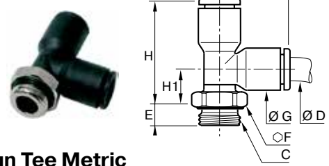
3193 Male Run Tee Metric Tube to Tube to Male BSP or M5
