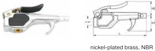
nickel-plated brass, NBR
