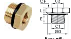
Brass with Bi-Material Seal
