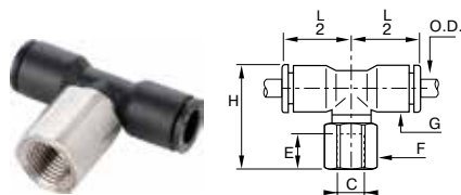
3008 Female Branch Tee Fractional Inch Tube to NPT
