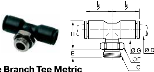
3198 Male Branch Tee Metric Tube to BSP or M5
