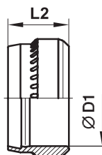
Bague progressive: PSR
