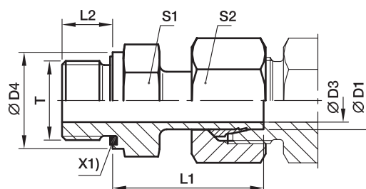
X1) Joint Eolastic ED
