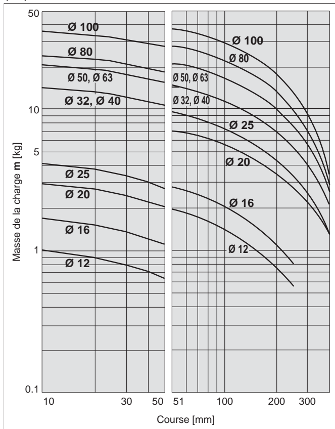
(13) L = 50 mm, V = 200 mm/s max.
