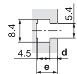
Dimensions de la rainure [mm]
