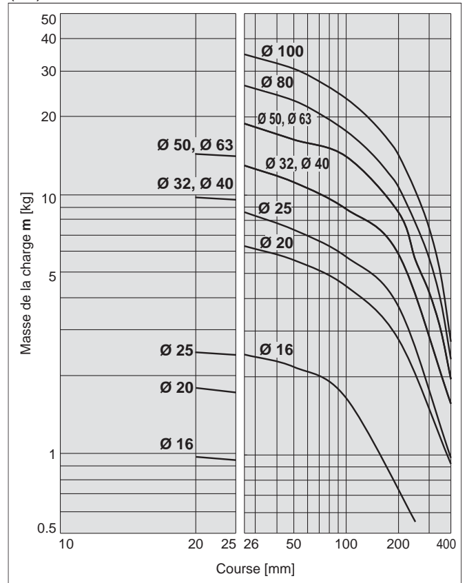
(16) L = 100 mm, V = 200 mm/s max.
