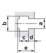
Dimensions de la rainure [mm]
