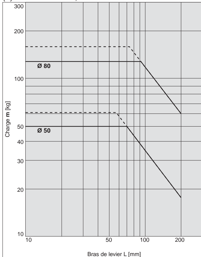
(3) Course max. 50, V = 400 mm/s
