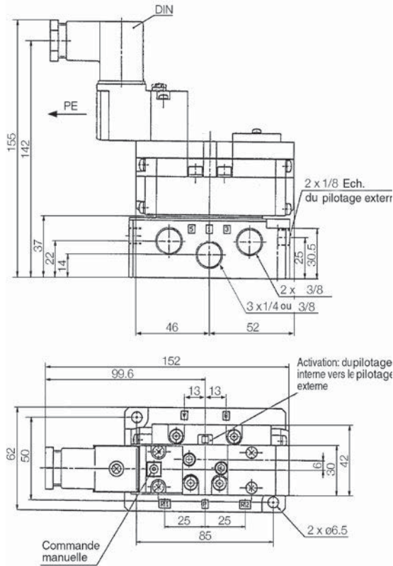
EVS7-6-FG-S-□CV-Q
