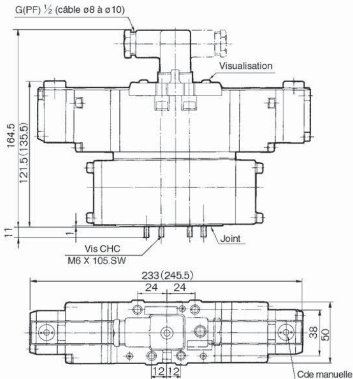
VS7-8-FPG-□□-Q
