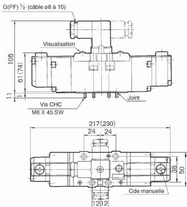
VS7-8-FG-D-□□-Q
