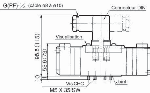
VS7-6-FG-D-□□-Q
