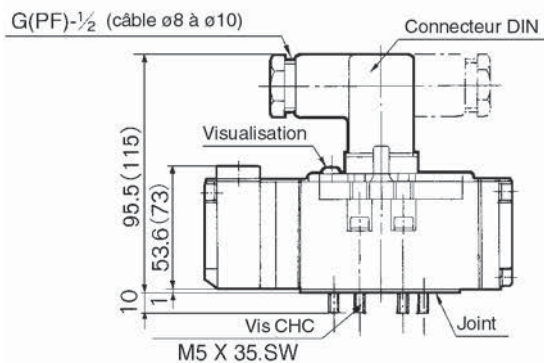
VS7-6-FG-S-□□-Q
