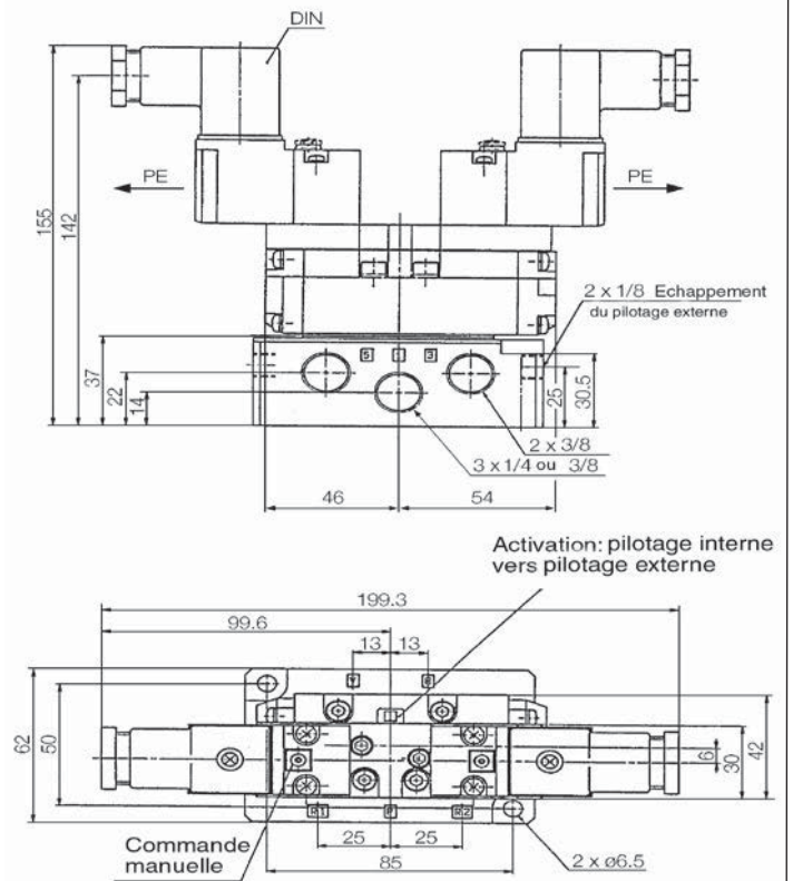
EVS7-6-FG-D-□CV-Q
