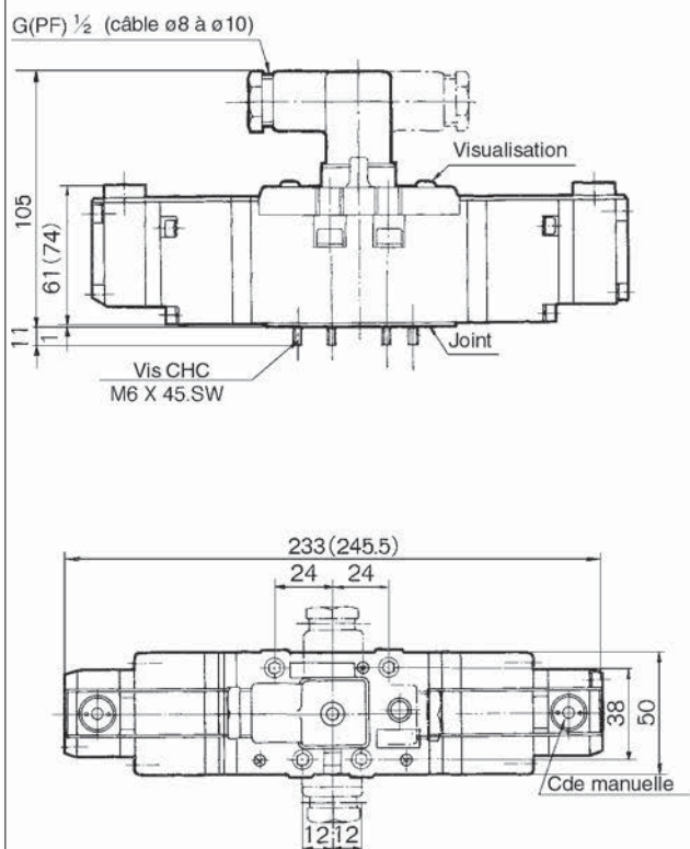
VS7-8-FHG-□□-Q VS7-8-FJG-□□-Q
