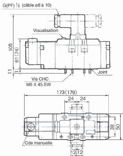
VS7-8-FG-S-□□-Q
