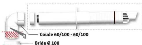
Kit Rolux Renofit® 60/100-60/100
