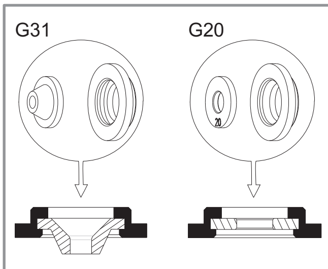
figure 32 - Diaphragme vanne gaz
