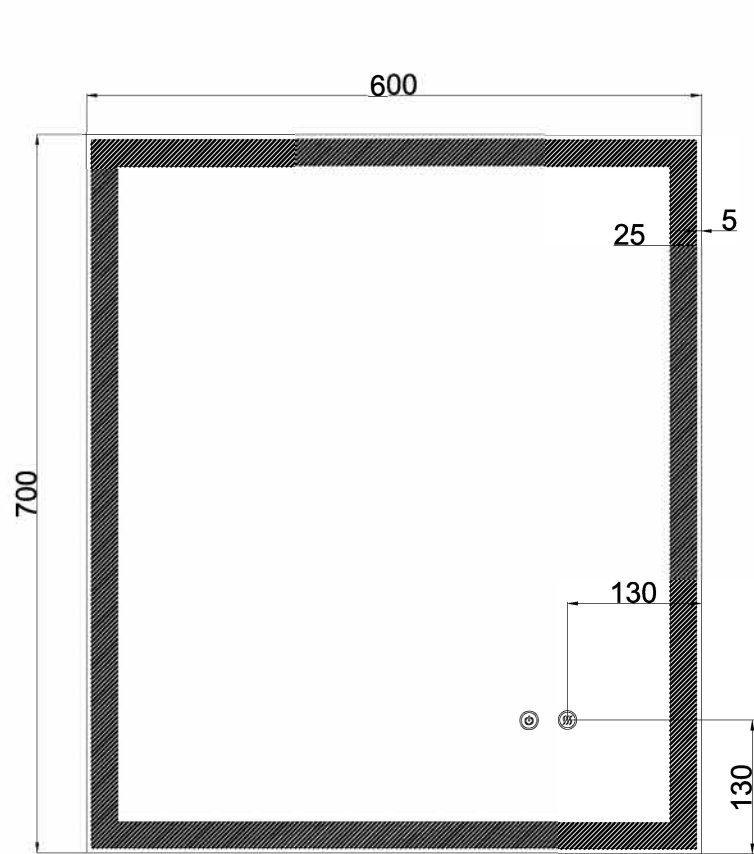
FRONT VIEW
