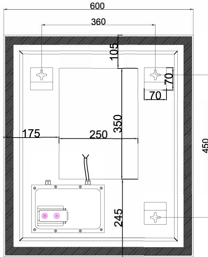
BACK VIEW
